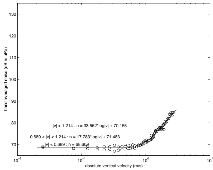
Figure 3-9: Band averaged noise model for the flow shield encased hydrophone attached to the SSAR bottom pressure case during the Aberdeen pond tests.
