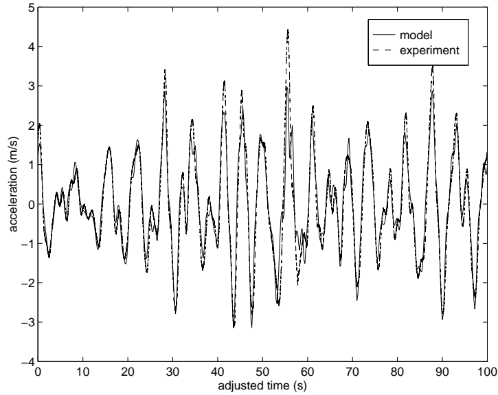
Figure 2-4: Comparison of accelerometer data from at-sea tests with model results generated by forcing the system with the actual surface motion from the at-sea test.
