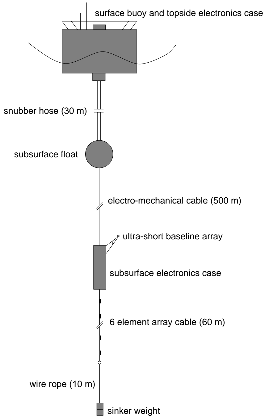
Figure 1-1: The current standard SSAR design.
