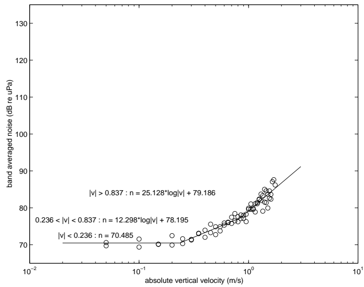
Figure 3-7: Band averaged acceleration equivalent noise model for a hydrophone attached to the SSAR array cable.
