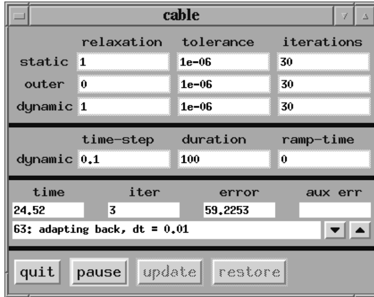
Figure 3.1: cable 's graphical information and control dialog.
